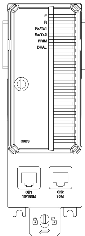
Figure 39. EtherNet/IP communication interface - CI873
