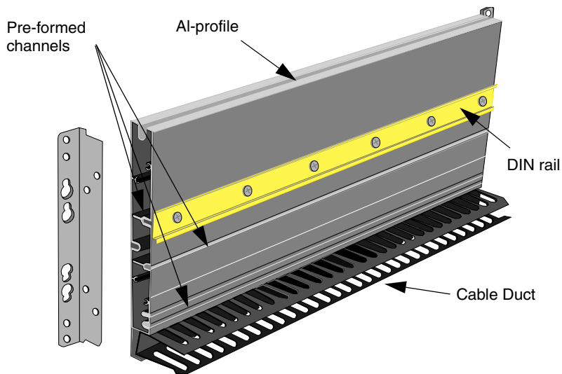
Figure 45. DIN Rail Mounted on an Al-Profile
