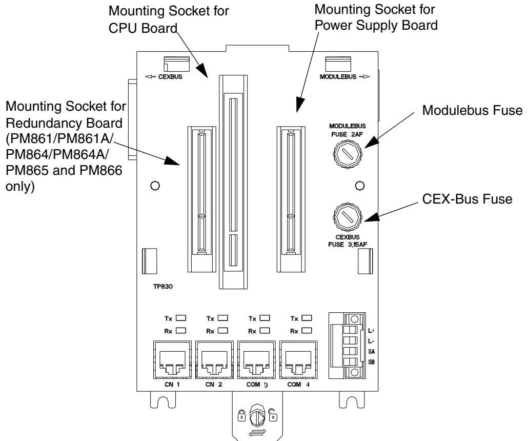
Figure 53. TP830 Base plate - Mounting Sockets and Fuses
