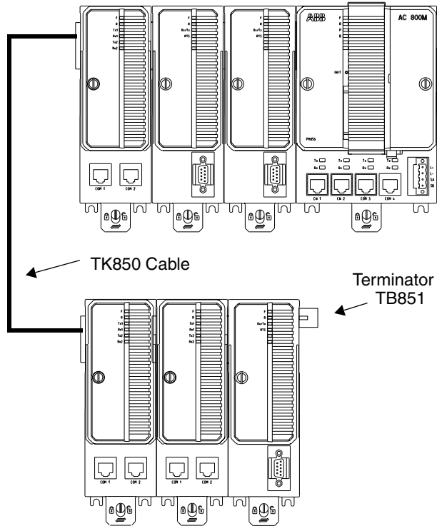
Figure 48. TB851 Terminator for CEX-Bus (Female)
