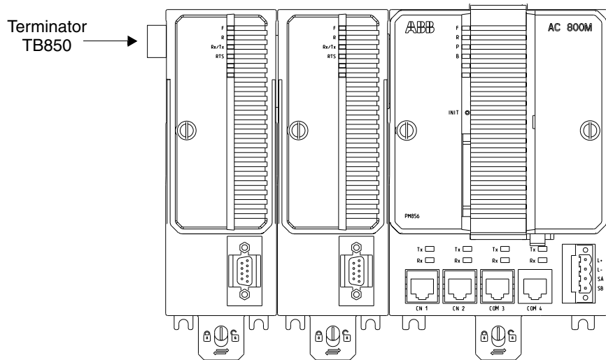
Figure 46. TB850 Terminator for CEX-Bus (Male)
