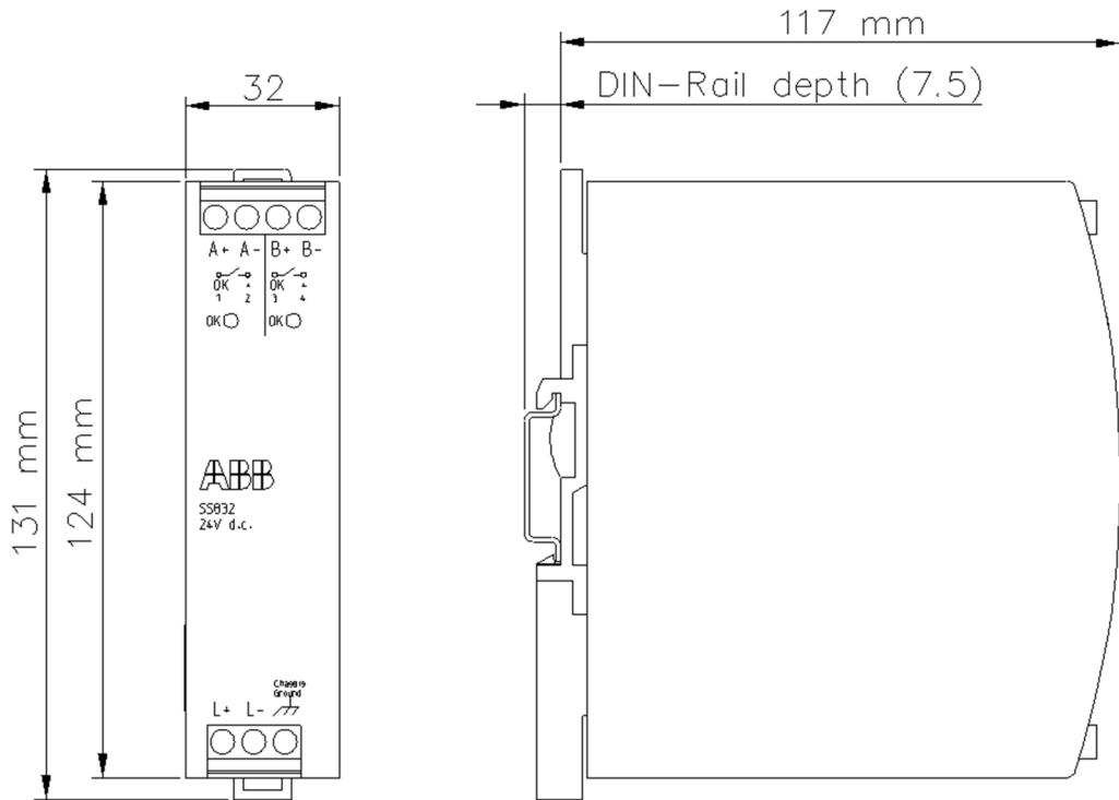
Figure 44. SS832 Voting Unit Dimensions and Connections
