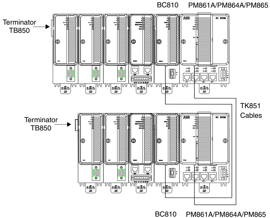
Figure 47. CEX-Bus Terminator when using Redundant Communication Interface Units (with BC810) and Controllers
